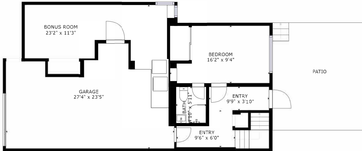
FLOOR 2
