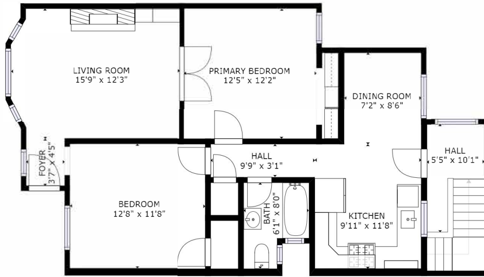
FLOOR 2
